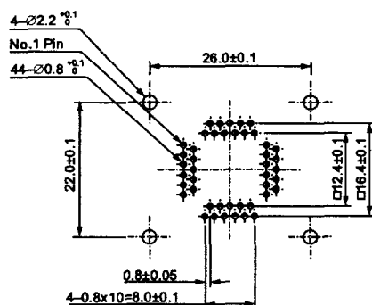
IC51-0444-798 (44 Pins)
