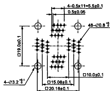
IC51-0484-806 (48 Pins)
