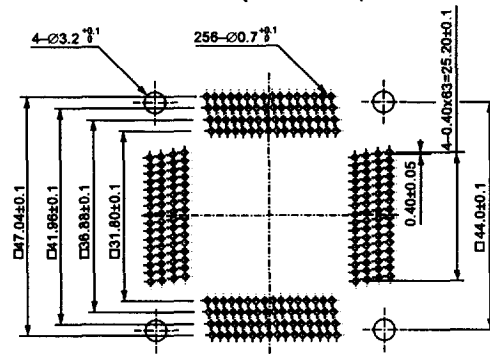
IC51-2564-1668 (256 Pins)
