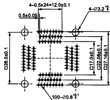
IC51-1004-809 (100 Pins)
