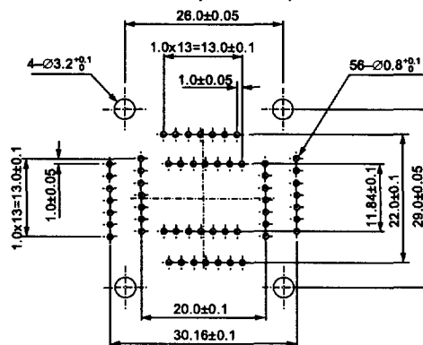
IC51-0564-790 (56 Pins)
