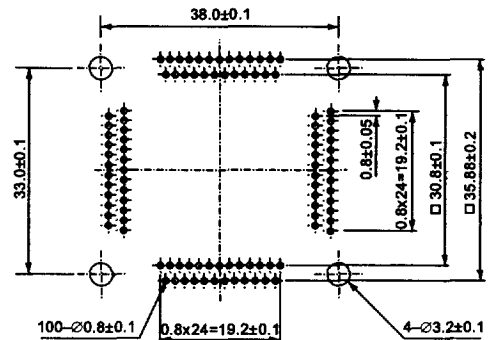
IC51-1124-1036-2 (112 Pins)
