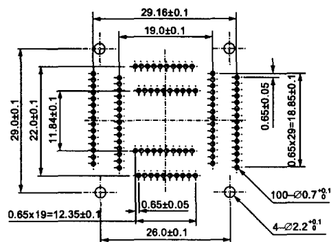
IC51-814-KS12033 (100 Pins)
